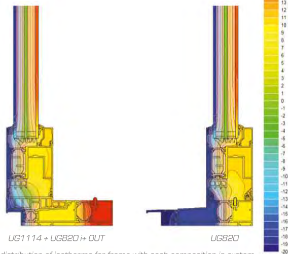
distribution of isotherms for frame with sash composition in system ULTRAGLIDE - low threshold option (UG 1114 + UG 820)
