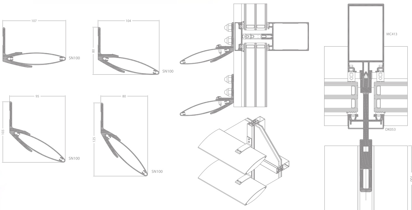
sample of dimensions and angles for Sun Protection panels
